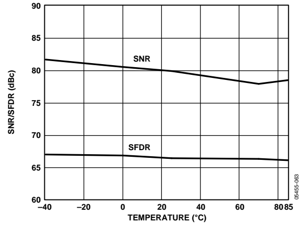
Figure 33. AD9237-65 SNR/SFDR vs. Temperature with f_{IN} = 32.5\text{MHz}
